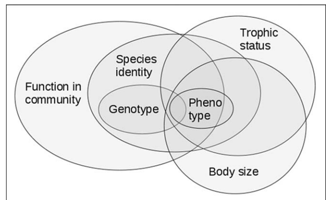
Fig. 2. Different types of aggregation can be nested such as phenotypes in species, body size and trophic status or may have no unique hierarchical structure such as in most other cases.
