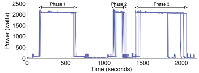
Figure 1: Superimposed power consumption traces of seven operation cycles of the same dishwasher appliance (data taken from [22]).
