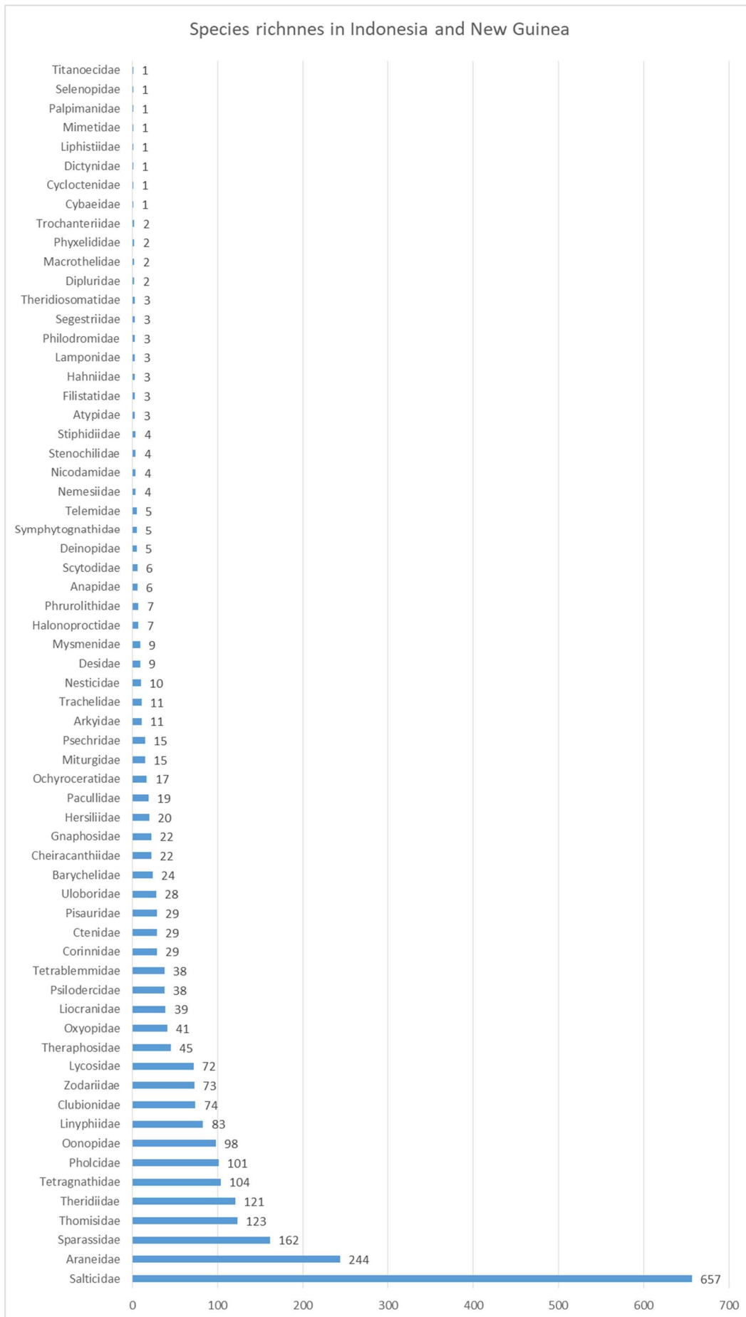
Figure 2. Number of species in families of spiders recorded for Indonesia and New Guinea
